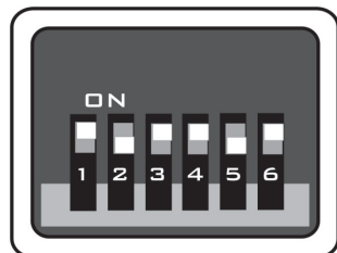
RS-701 DIP Switches
